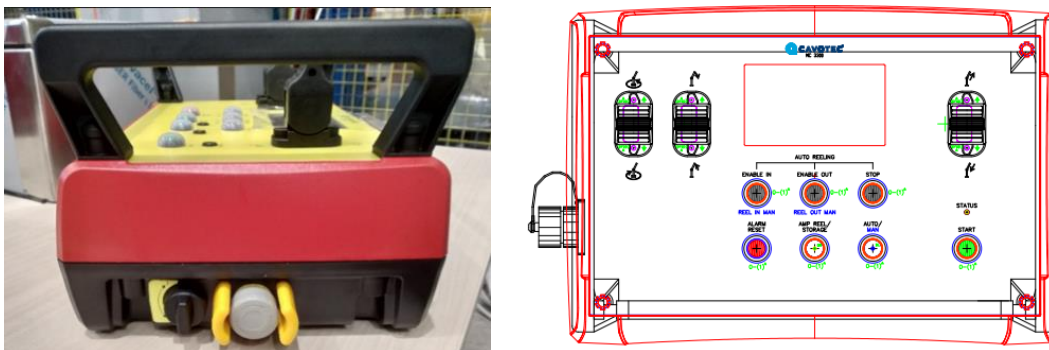
Figura 45. Control remoto
